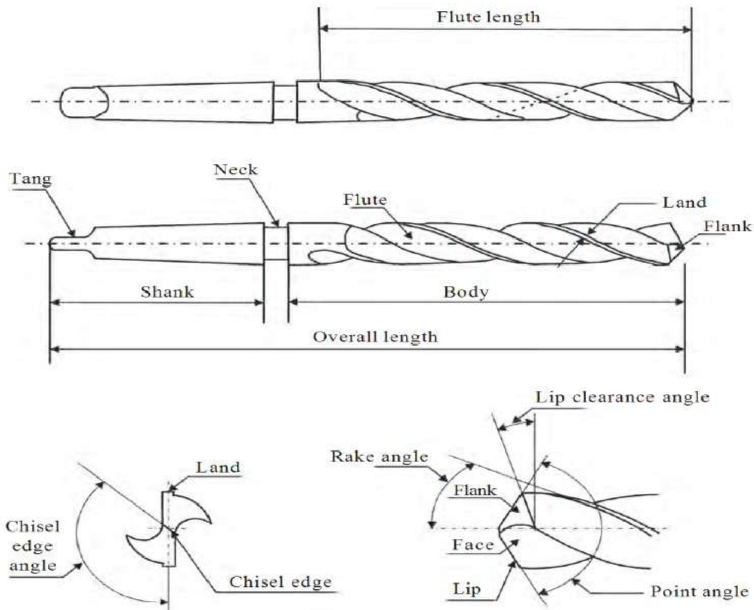
Twist drill nomenclature
